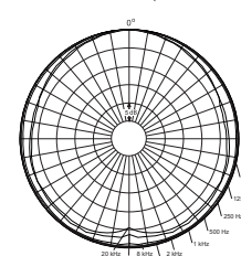
Polar Pattern (normalized, all except SC4071 & SCO71-H)
