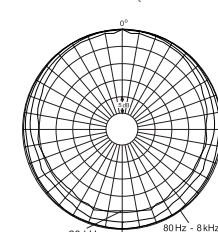
Polar Pattern (normalized, SC4071 & SCO71-H)
