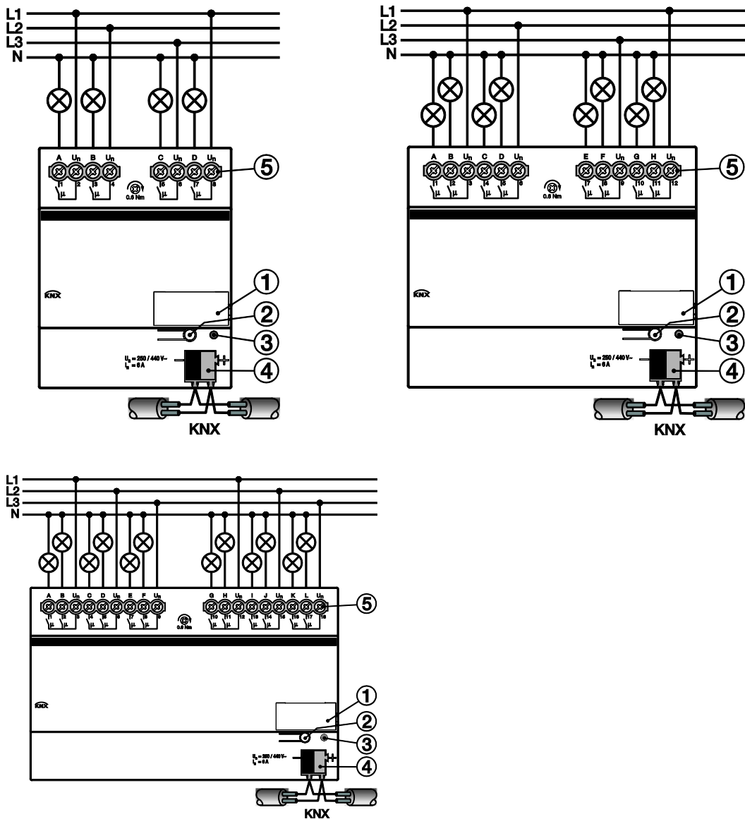
Connection schematic SA/S x.6.1.1
