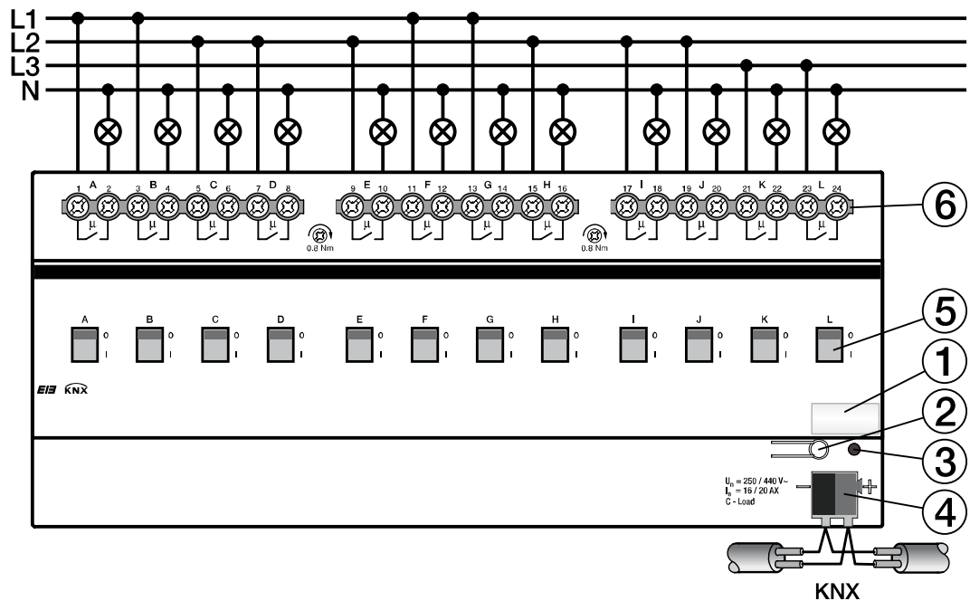
Connection schematic SA/S x.16.6.1
