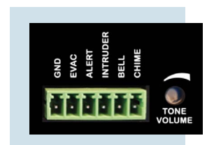
5 Tone Generator
