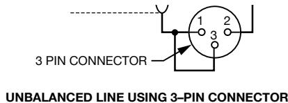
UNBALANCED LINE USING 3-PIN CONNECTOR
